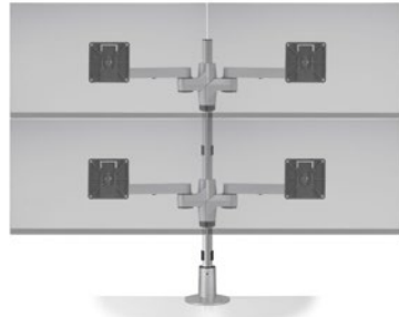
STAXX TWO OVER TWO Screen Size: Up to 24" Weight Capacity: Up to 15 lbs. per monitor Part Number: STX-22S-___
