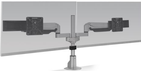
E2 CONNEX DYNAMIC DUAL WIDE Screen Size: Up to 39" (bezel measured left to right) Weight Capacity: 2.2 - 20 lbs. per monitor Part Number: E2-02-SD-__ _
