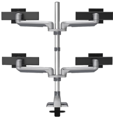
E5 TWO OVER TWO STATIC POLE Screen Size: Up to 27" Weight Capacity: 0-15 lbs. per monitor Part Number: E5G-P22S-__
